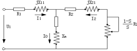
Fig. F1-1 Steady State Equivalent Circuit of Asynchronous Motor
