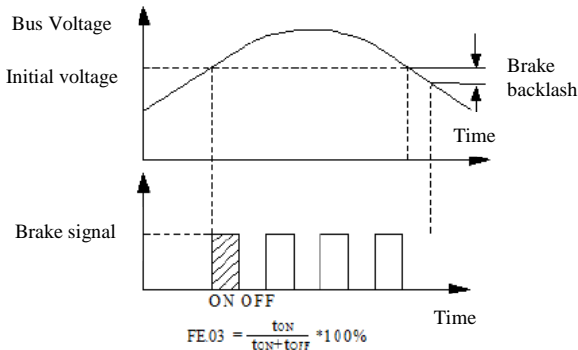
Fig. FE-1 Dynamic Braking
