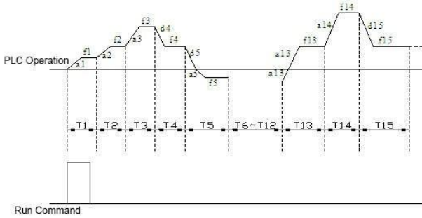
Fig.FC-2 Maintain Last Stage after Single Cycle
