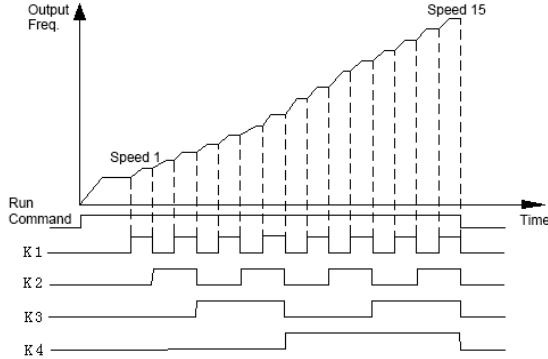
Figure F7-1 Multi-speed Running
