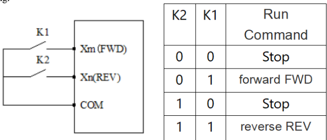
Fig. F4-3 2-wire Control Mode 2
