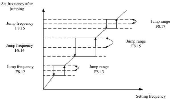
Fig. F8-2 Hopping Frequency
