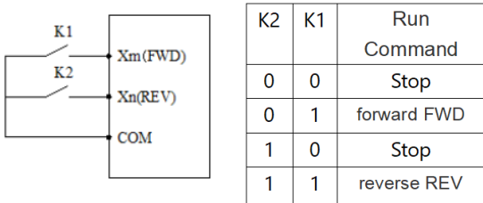
Fig. F4-2 2-wire Control Mode 1
