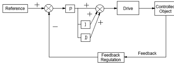
Fig. FA-1 Analog Feedback Control System
