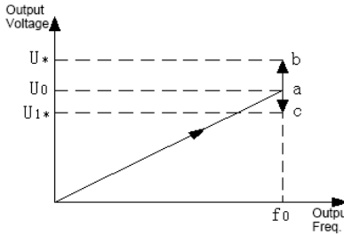
Fig. F3-4 Voltage Control Mode 0
